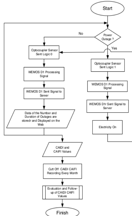
Figure 7. Flowchart of Power Outages Sensing Device
