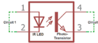
Figure 3. Optocoupler Configuration [7]
