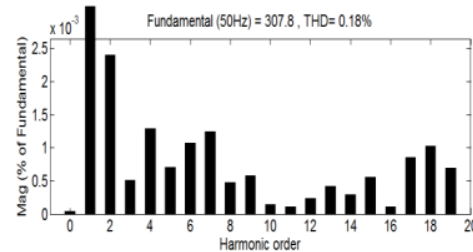
(f) With double tuned filter (irradiance 1000 W/m 2 )
