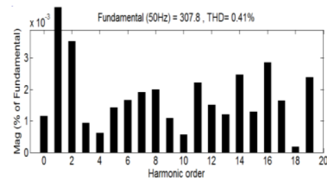
(d) With single tuned filter (irradiance 1000 W/m 2 )
