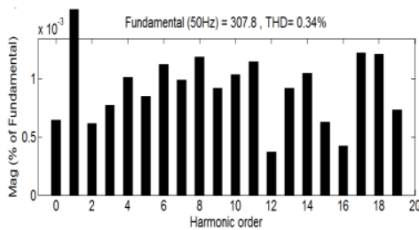
(c) With single tuned filter (irradiance 600 W/m 2 )
