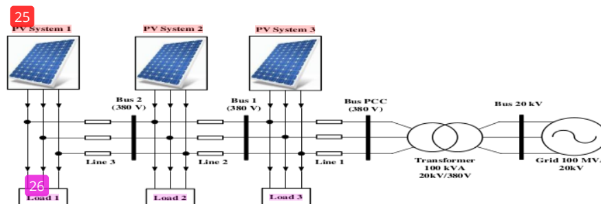
Figure 2. Proposed model of multi units of PV generator connected to three phase grid
