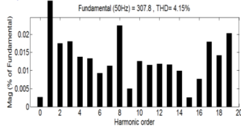
(b) Without filter (irradiance 1000 W/m 2 )
