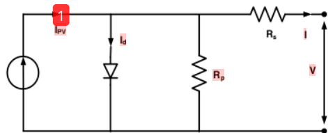
Figure 3. Equivalent circuit of solar panel
