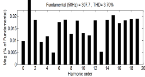
(a) Without filter (irradiance 600 W/m 2 )
