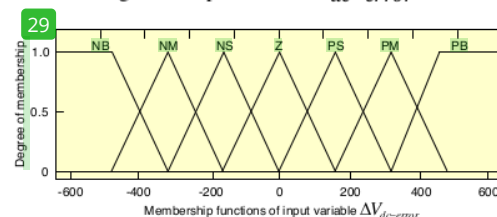
Figure 8 Input MFs of \Delta V_{dc-error}
