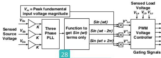
Figure. 4 Series active filter control
