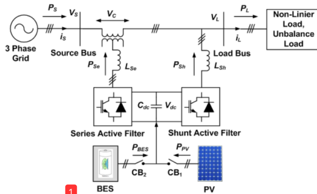
Figure. 2 Active power transfer using UPQC-PV-BES system
