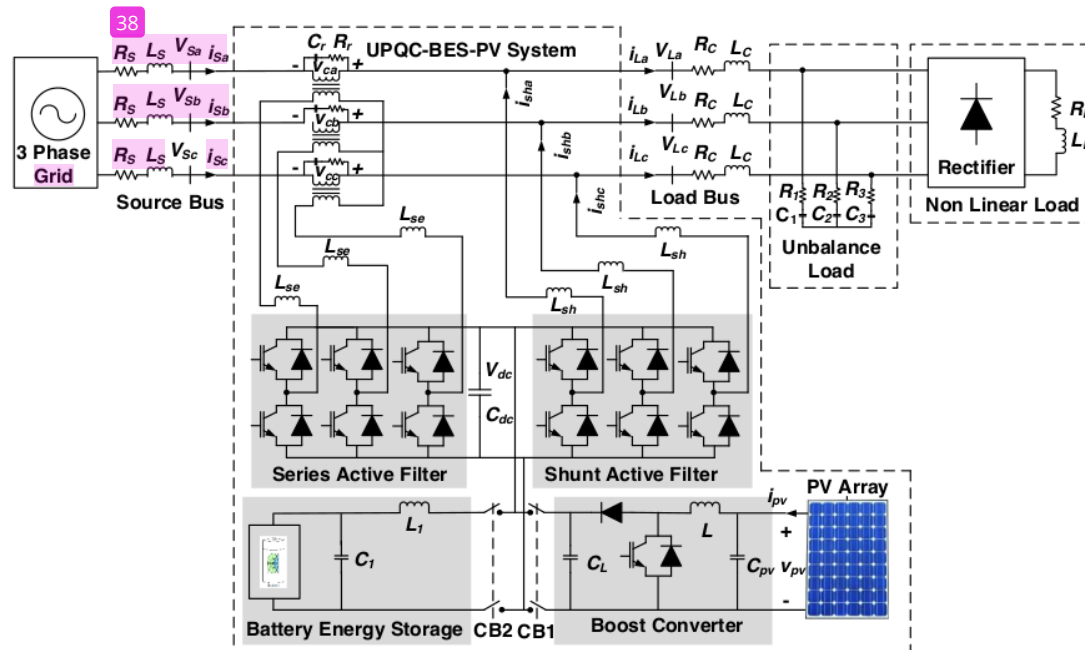
Figure 1 Proposed model using UPQC-PV-BES
