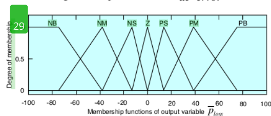
Figure 9 Output MFs of \bar{p}_{loss}
