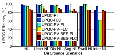
Figure 17 Efficiency of UPQC combinations
