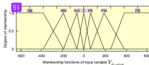
Figure 7 Input MFs of V_{dc-error}
