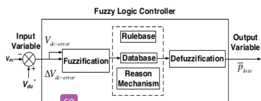
Figure 6 Block diagram of FLC
