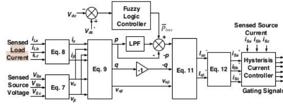
Figure. 5 Shunt active filter control
