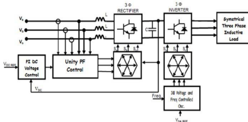
Figure 1. Proposed of AC-AC converter
