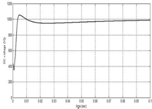
Figure 26. DC voltage, case 6
