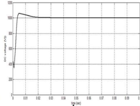
Figure 18. DC voltage, case 4
