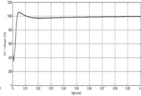
Figure 6. DC voltage, case 1
