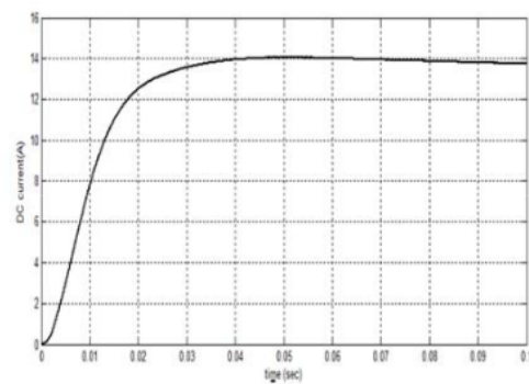
Figure 25. DC current, case 6
