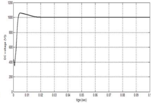
Figure 22. DC voltage, case 5
