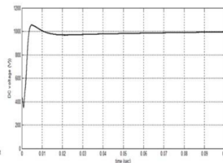
Figure 10. DC voltage, case 2
