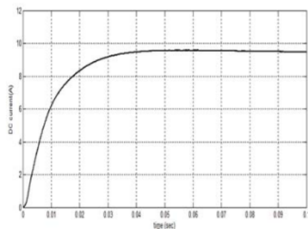
Figure 9. DC current, case 2
