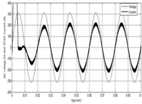
Figure 11. Amplitude of voltage and current at iinput of rectifier, case 2
