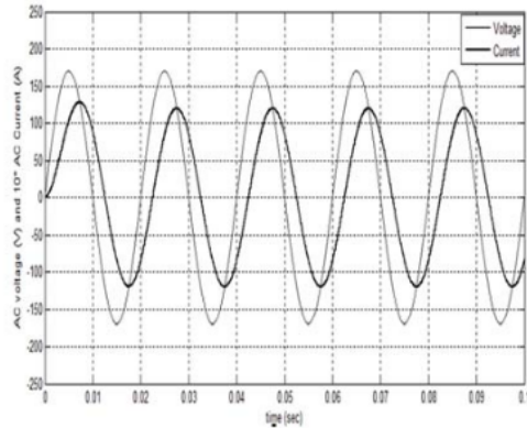
Figure 20. Amplitude of voltage and current at output of inverter, case 4
