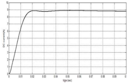
Figure 5. DC current, case 1
