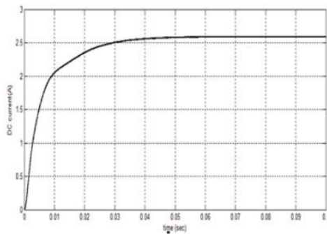
Figure 13. DC current, case 3
