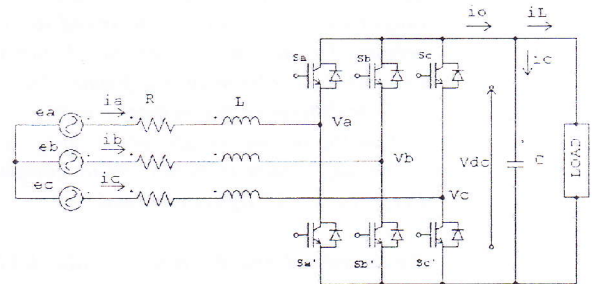
Fig. 2. The topology of the three-phase active rectifier system
