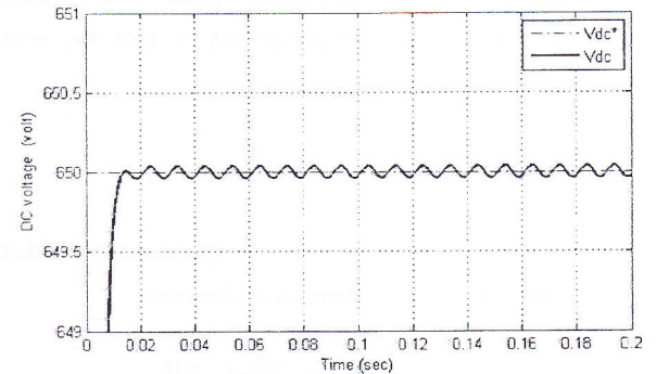
Fig. 9(b). The DC voltage under the unbalance condition
