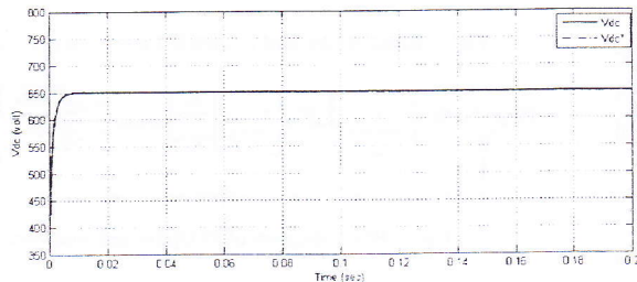
Fig. 7(b). The DC voltage with feedback linearization
