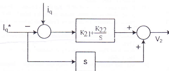
Fig. 4. Block diagram of power factor control
