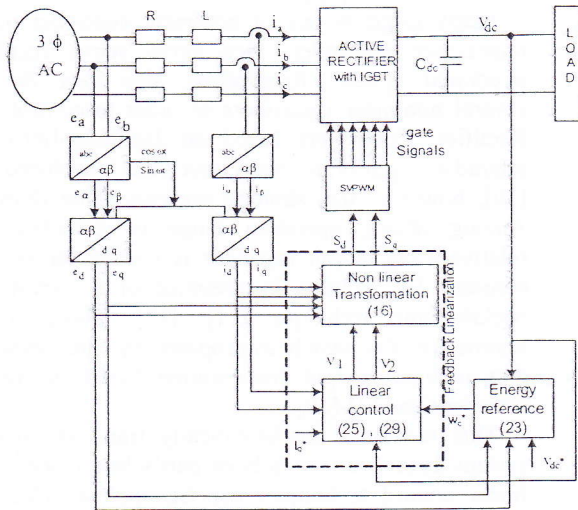
Fig. 1. Block Diagram of the Proposed Control Strategy
