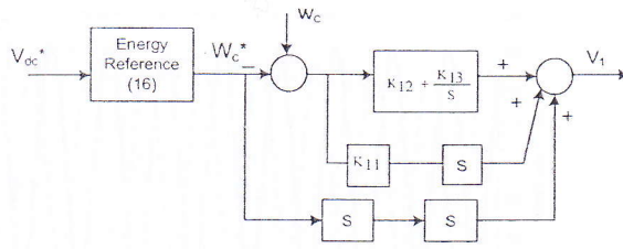
Fig. 3. Block diagram of the DC voltage control
