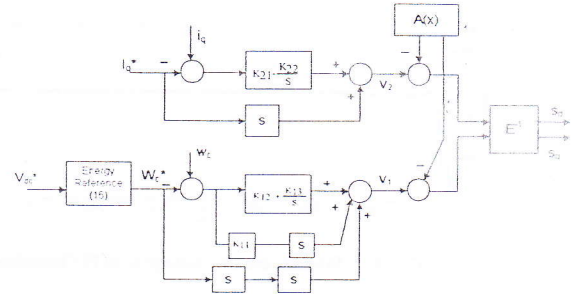
Fig. 5. Block diagram of Feedback Linearization Control
