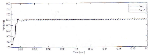
Fig. 7(a). Presents the DC voltage with PI Optimized
