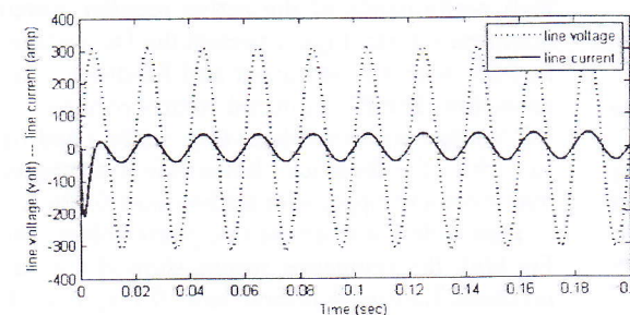
Fig. 8(b). Demonstrates the line phase voltage and current of the proposed control
