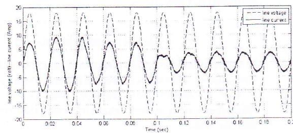
Fig. 8(a). Demonstrates the line phase voltage and current of PI optimized
