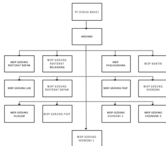
Figure 3.4 Transmission Block Diagram
