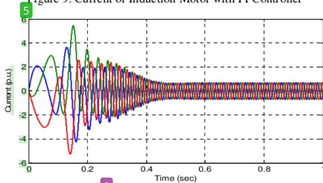
Figure 10. Current of Induction Motor with Fuzzy-PI Controller
