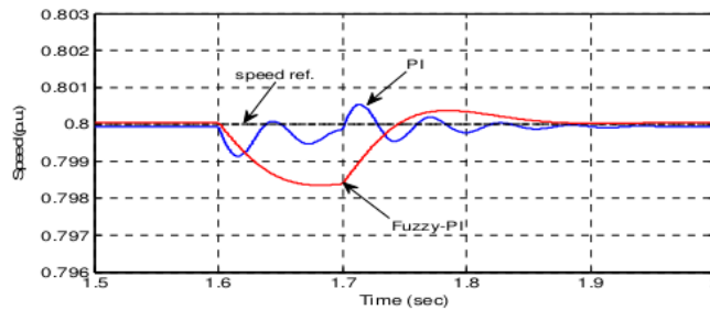
Figure 14. Speed responses for disturbance condition
