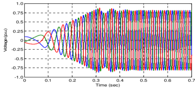
Figure 11. Voltage of Induction Motor with PI Controller
