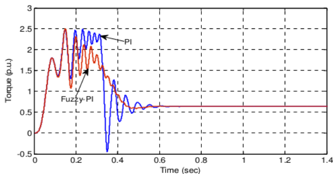
Figure 8. Electromagnetic torque response for normal condition
