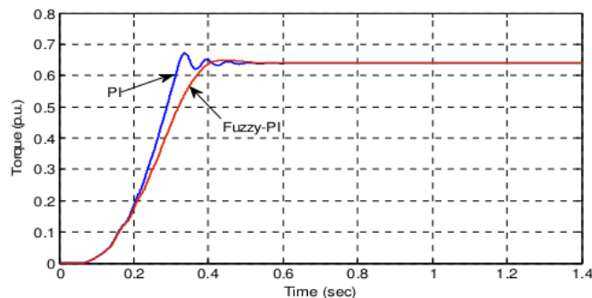
Figure 7. Load torque for normal condition
