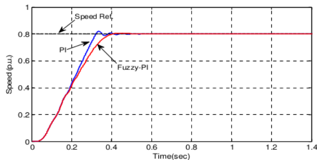
Figure 6. Speed response for normal condition
