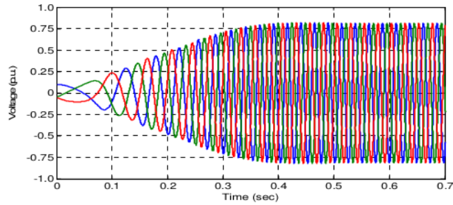
Figure 12. Voltage of Induction Motor with Fuzzy-PI Controller
