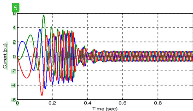
Figure 9. Current of Induction Motor with PI Controller
