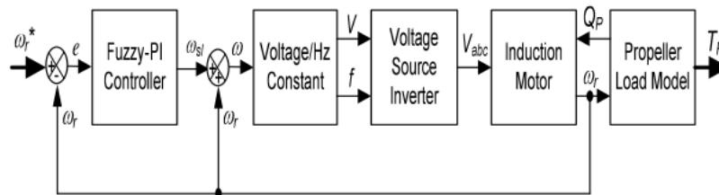
Figure 5. Block diagram of simulation model
