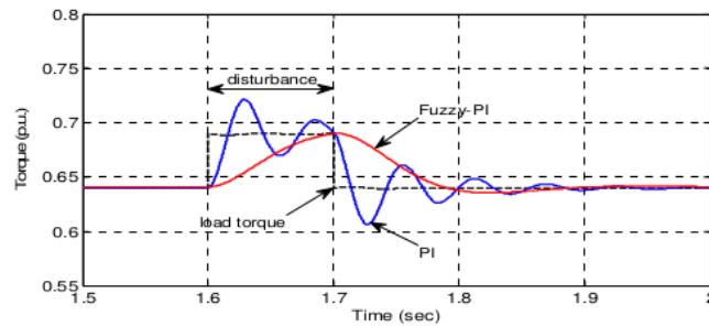
Figure 13. Electromagnetic torque for disturbance condition
