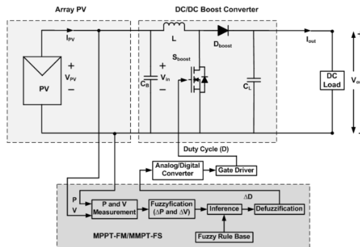
Figure. 2 PV system using MPPT-FM/MPPT-FS method connected to DC load
