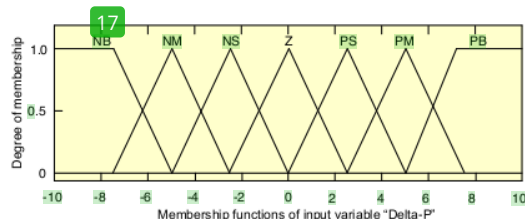
Figure. 7 Input MFs of MPPT-FM/MPPT-FS ( \Delta P )
