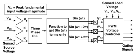
Figure. 4 UVTG control of series active filter
