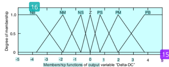
Figure. 8 Output MFs of MPPT-FM ( \Delta D )
