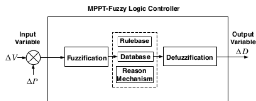
Figure. 5 MPPT-fuzzy Mamdani/MPPT fuzzy Sugeno
