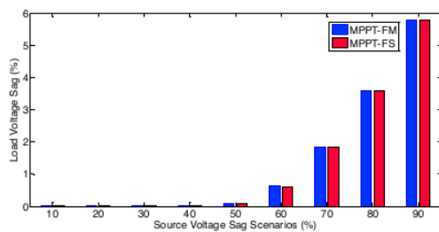
Figure. 14 Percentage of load voltage sag
