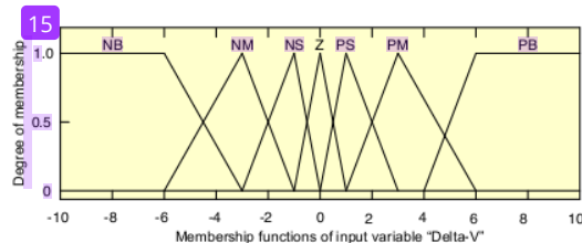
Figure. 6 Input MFs of MPPT-FM/MPPT-FS ( \Delta V )
