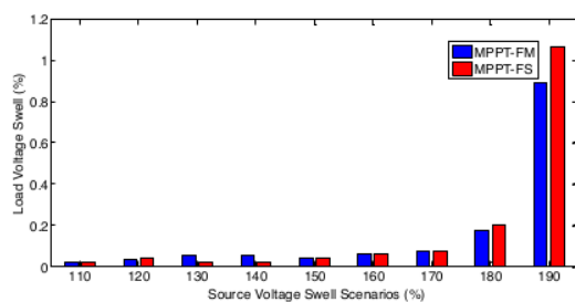
Figure. 15 Percentage of load voltage swell
