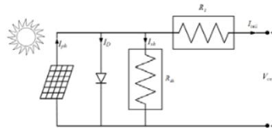
Figure 5. Equivalent Circuit of PV Cell
