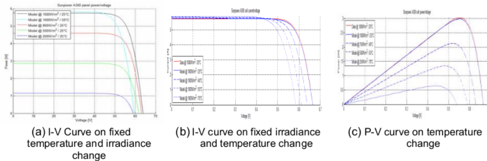
Figure 4. Characteristic Curve of Panel PV (Type MSX-60)
