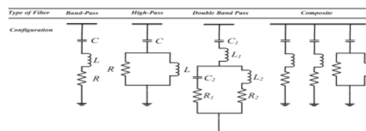
Figure 6. Models of Passive Filter
