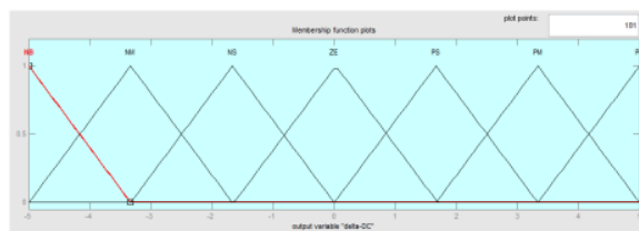
Figure 10. Output Variable Duty Cycle Change (Delta D)
