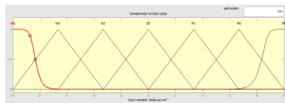
Figure 9. Input Variable Power Change (Delta Power)
