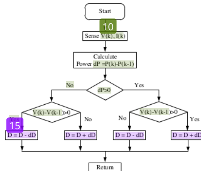
Figure 4. P and O Algorithm
