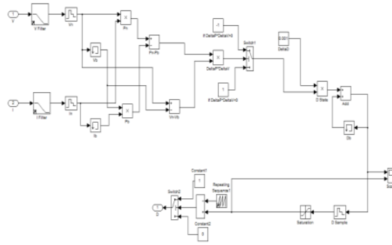
Figure 5. Matlab/Simulink Model for MPPT Using P and O Algorithm
