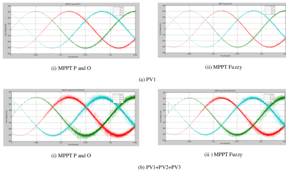
Figure 11. Simulation Results of Grid Voltage on Two Models of PV Generator Integration Connected to Three Phase Grid Under Solar Irradiance 1000 W/m 2 on PCC Bus
