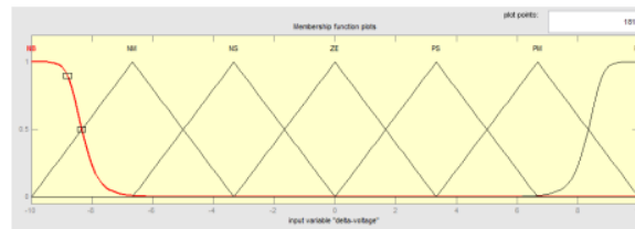
Figure 8. Input Variable Voltage Change (Delta Voltage)
