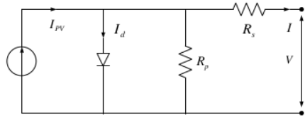
Figure 3. Equivalent Circuit of Solar Panel
