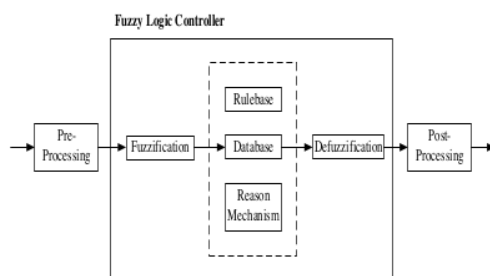
Figure 6. Blok Diagram of Fuzzy Logic Controller
