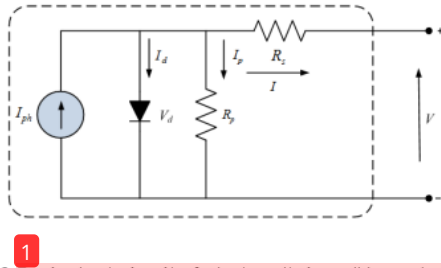
Figure 2 Equivalent circuit of photovoltaic cell based on single diode model
