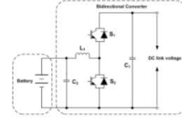
Figure 5 Model of battery energy storage
