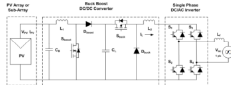
Figure 6 Single Phase PV Generator Model
