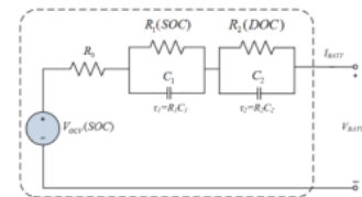
Figure 4 Equivalent circuit of 2nd order Randle model
