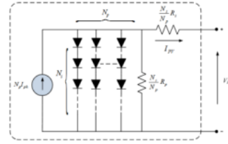
Figure 3 Electrical equivalent of solar array circuit
