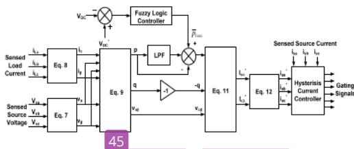
Fig. 4. Control strategy of shunt active filter
