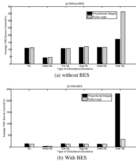
Fig. 11. Performance of average THD of source current of UPQC supplied by PV using PI and FLC in six disturbance scenarios
