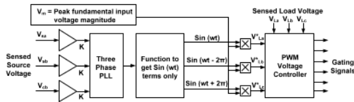
Fig. 3. Control strategy of series active filter
