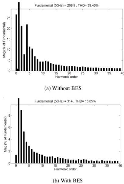
Fig. 9. Spectra of load voltage harmonics on phase A UPQC supplied PV using FLC in Scenario 6 (Inter-NL)
