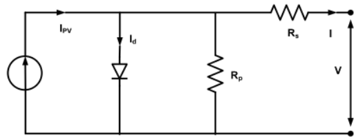
Fig. 2. Equivalent circuit of solar panel
