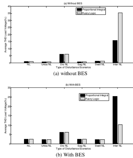
Fig. 10. Performance of average THD of load voltage of UPQC supplied by PV using PI and FLC in six disturbance scenarios
