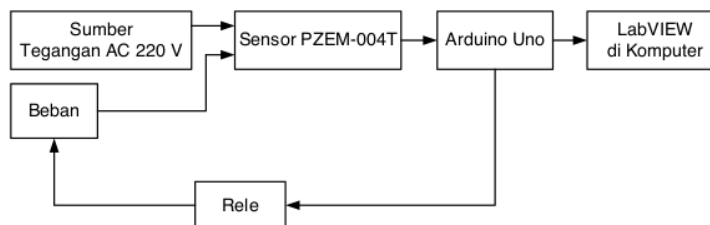
Gambar 2. Blok Desain Hardware Sistem Monitoring
