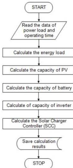
Figure 2. Research methodology for design of solar power plant.
