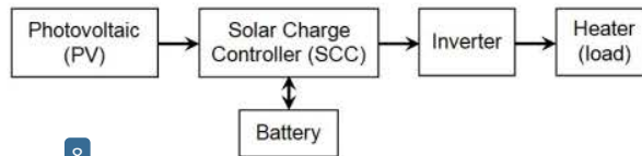
8 Figure 1. The block diagram of the solar power plant.
