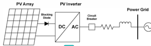
Figure 4. Proposed model for grid-connected photovoltaic system
