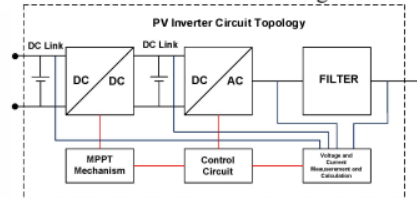
Figure 6. PV inverter circuit topology
