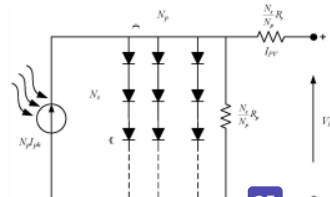
Figure 5. Equivalent circuit of PV array
