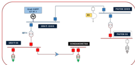
Figure 3. Power and Voltage Delivery Lines in Schematic 1
