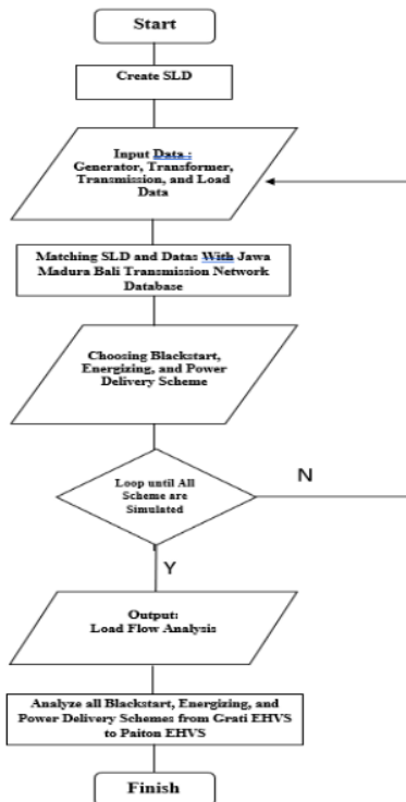
Figure 11. Flowchart of Schematic Modeling on DigSILENT
