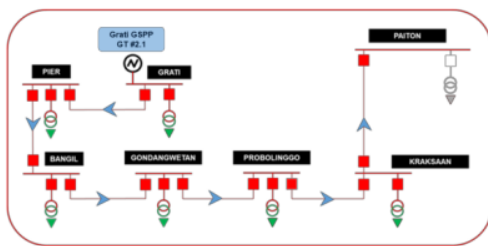
Figure 6 Power and Voltage Delivery Lines in Schematic 4
