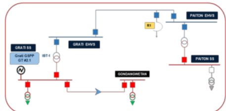
Figure 4. Power and Voltage Delivery Lines in Schematic 2
