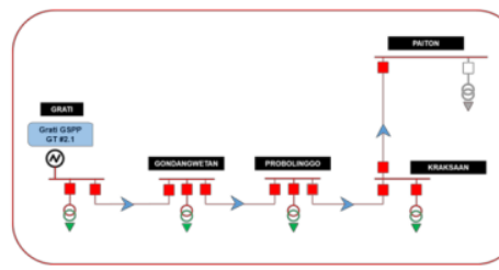
Figure 10. Power and Voltage Delivery Lines in Schematic 8
