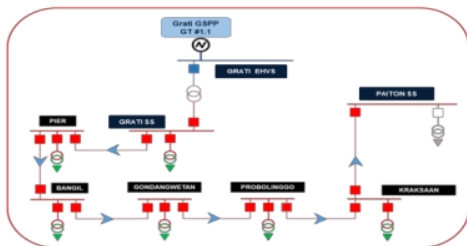
Figure 5. Power and Voltage Delivery Lines in Schematic 3
