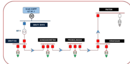
Figure 9. Power and Voltage Delivery Lines in Schematic 7.
