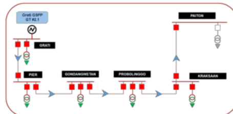
Figure 8. Power and Voltage Delivery Lines in Schematic 6.
