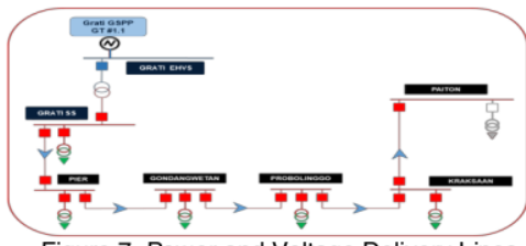
Figure 7. Power and Voltage Delivery Lines in Schematic 5
