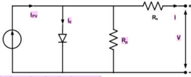
Fig. 2. Equivalent circuit of solar panel
