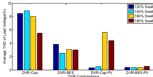
Fig. 11. Performance of average THD load voltage for voltage swell
