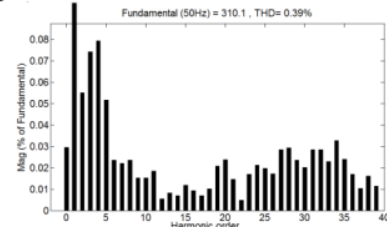
Fig. 8. THD load voltage on phase A for 60% sag
