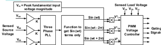
Figure 3. UVTG control of series active filter
