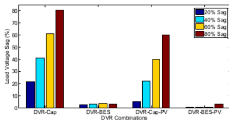
Fig. 6. Percentage of load voltage sag
