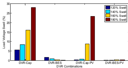
Fig. 7. Percentage of load voltage swell
