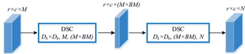
Fig. 3 – Depthwise Separable Convolution Bottleneck with Expansion (DSC-BE).
