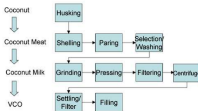
Fig 1. Virgin Coconut Oil Production Process
